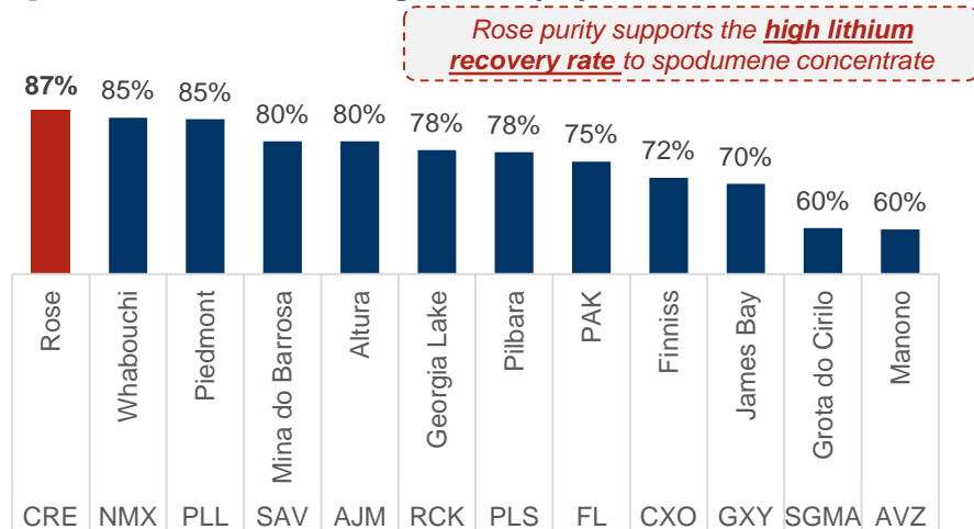
Spodumene Recovery Rate (%)
