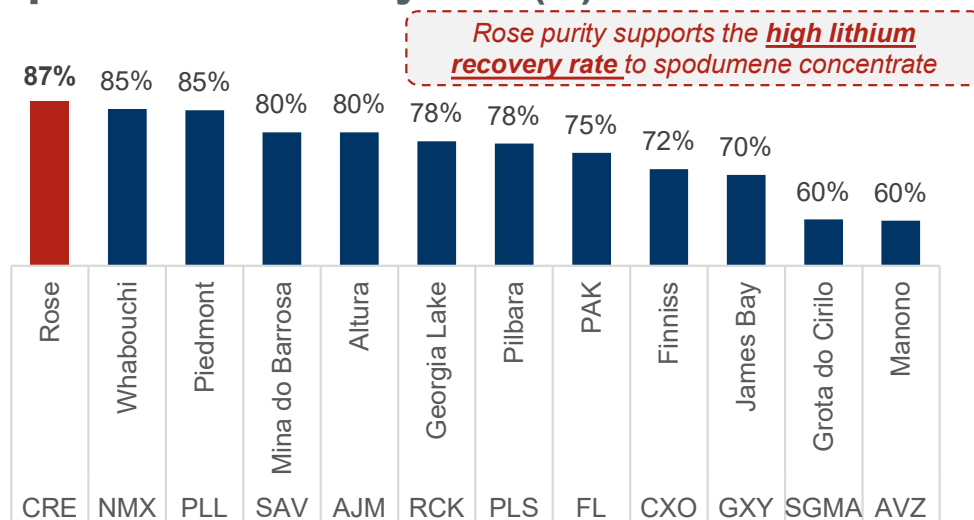
Spodumene Recovery Rate (%)
