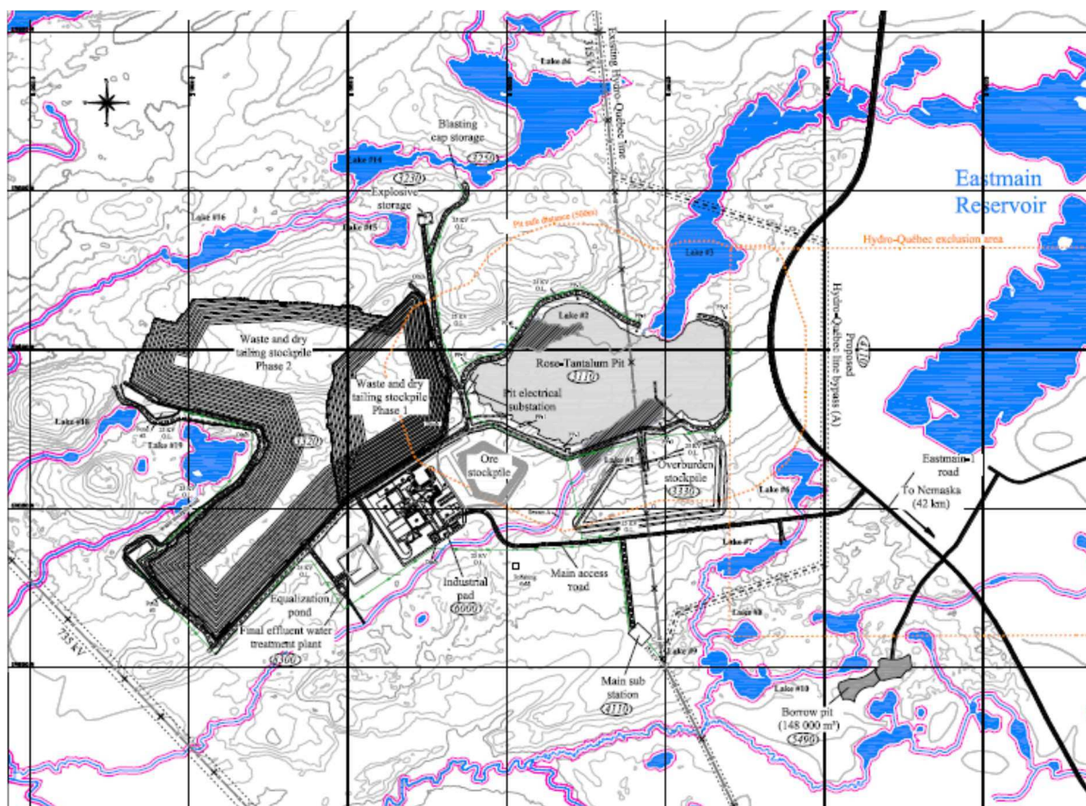
Figure 5 – Plan du site Rose lithium-tantale
