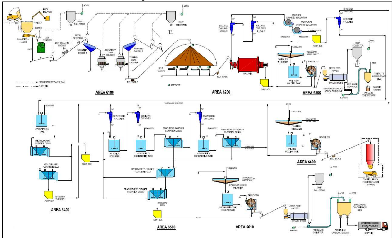
Figure 4: Process Flowsheet
